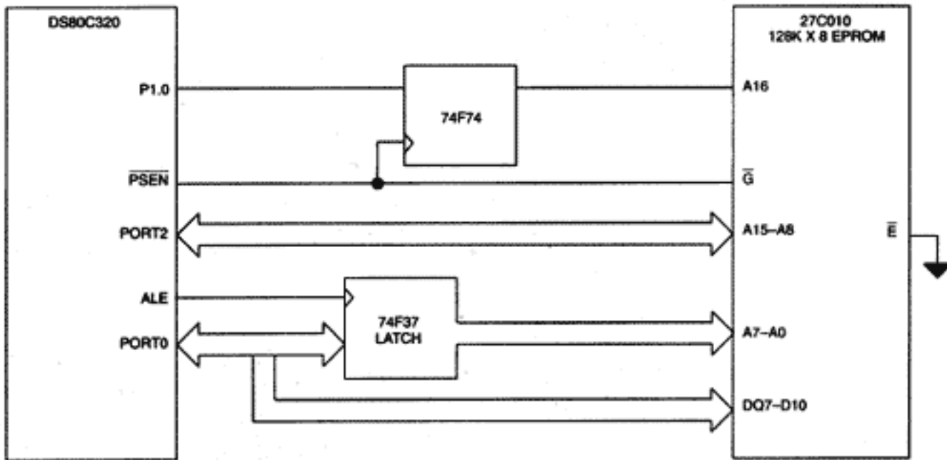
Figure 1. Simple Page Expansion Example Hardware
