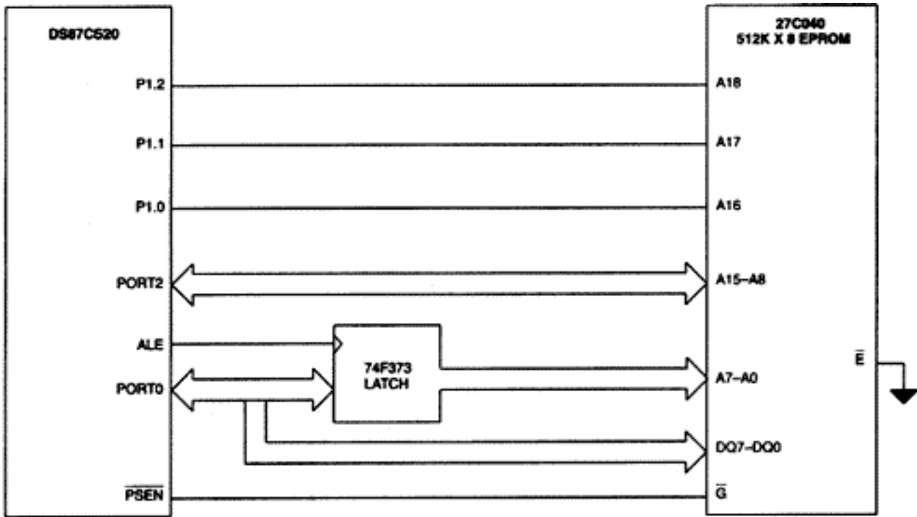
Figure 8. ROMSIZE Feature Common-Page I/O Expansion
