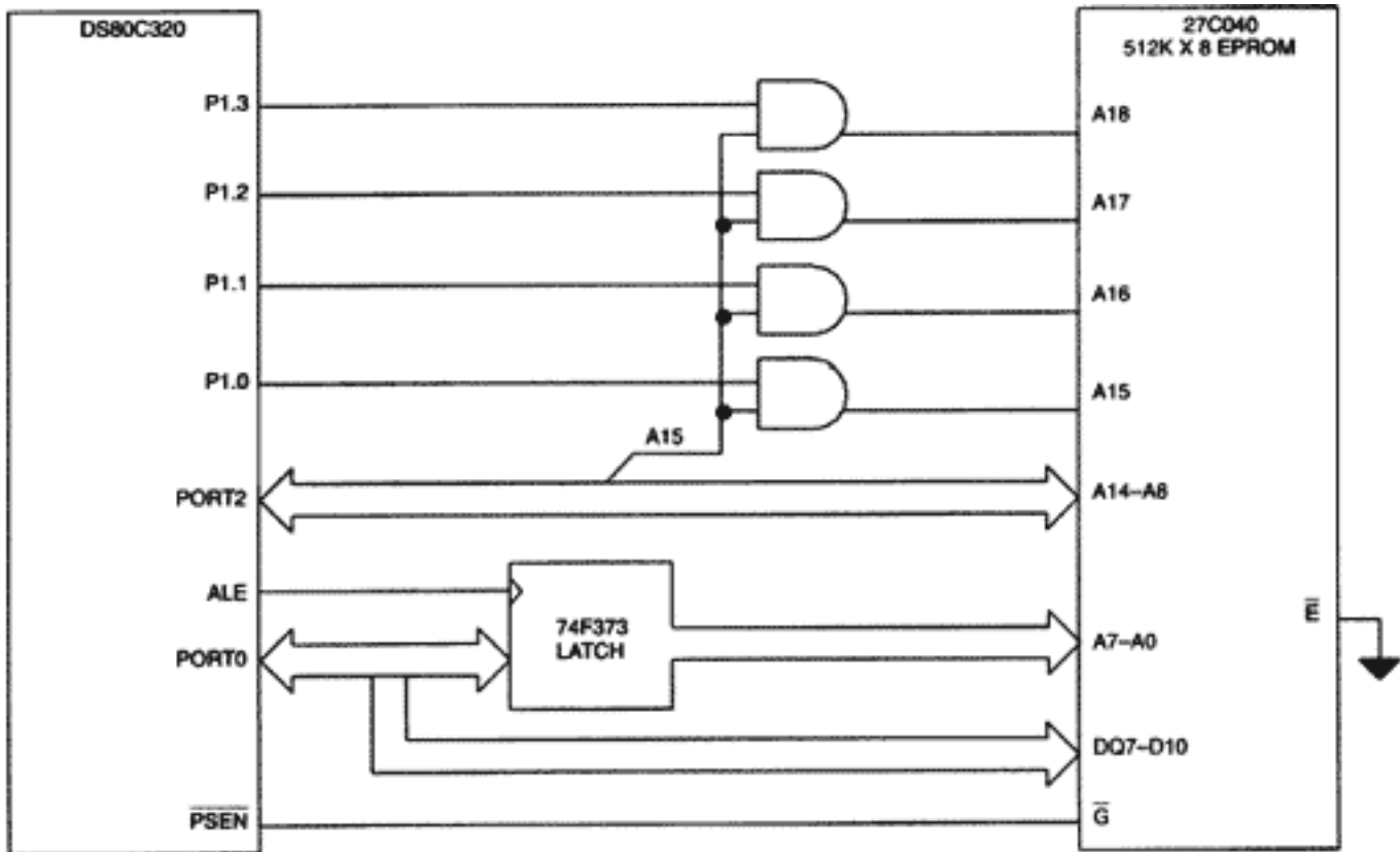
Figure 5. DS80C320 Expanded Memory Example Hardware Configuration
