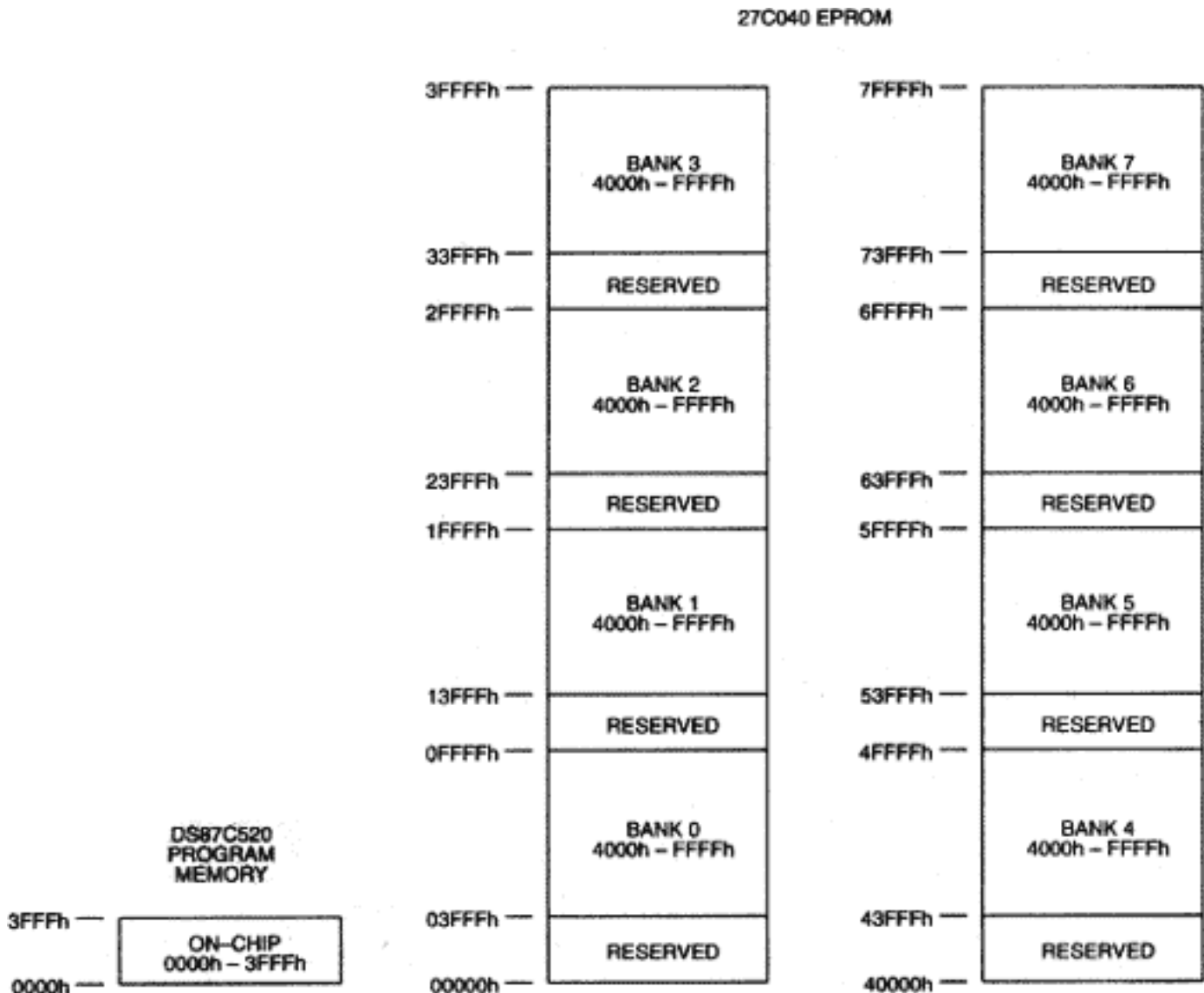
Figure 7. ROMSIZE Feature Common-Page Expansion Memory Map
