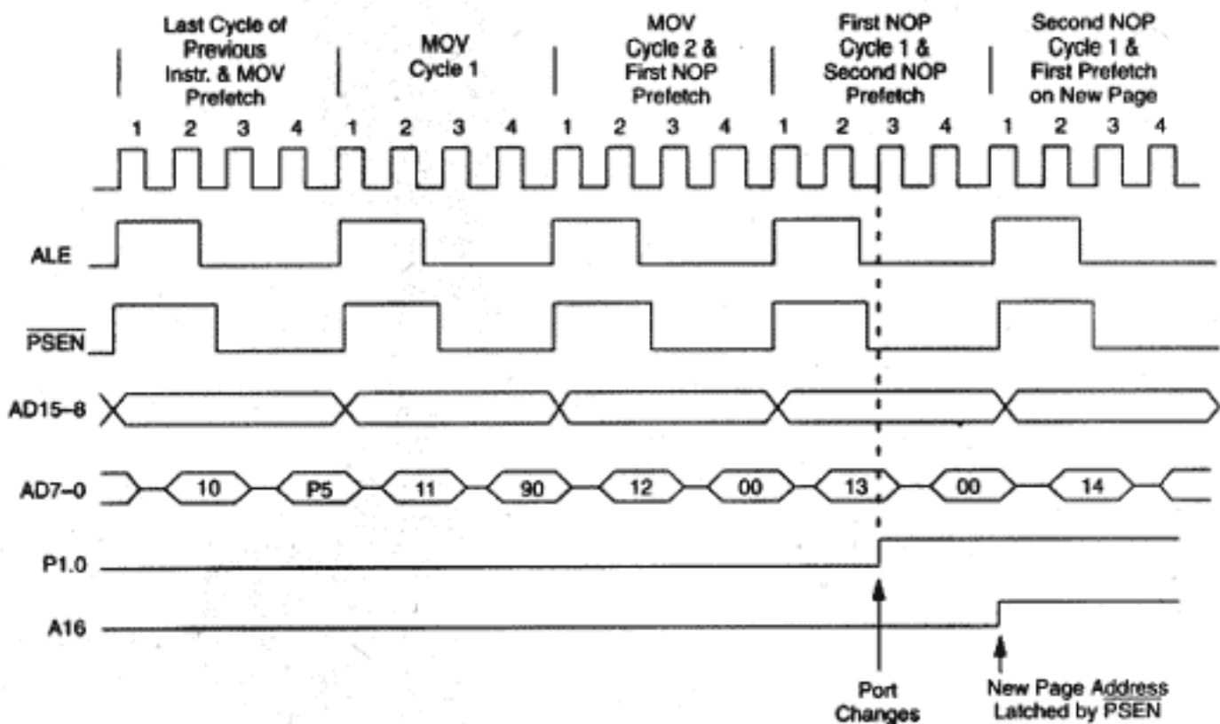
Bank Switching Timing Diagram
