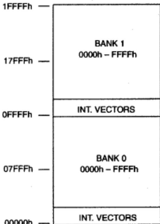
Figure 2. Simple Page Expansion Example Memory Map
