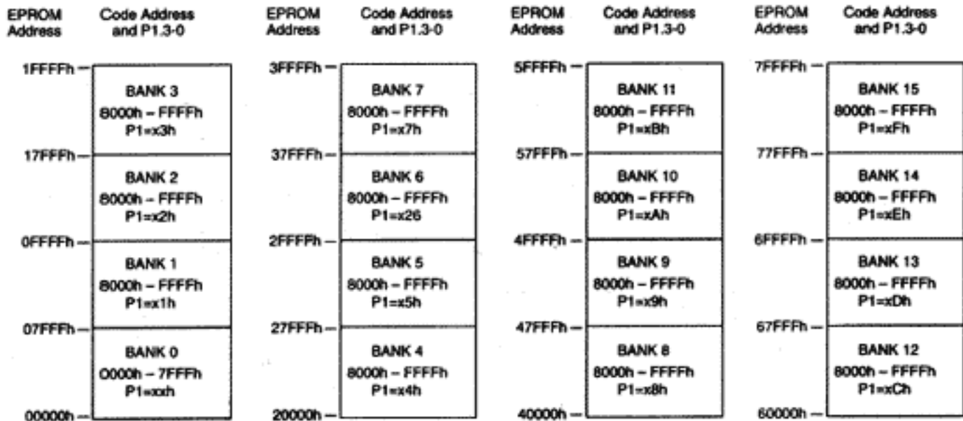
Figure 4. Common-Page Expansion Memory Example Memory Map
