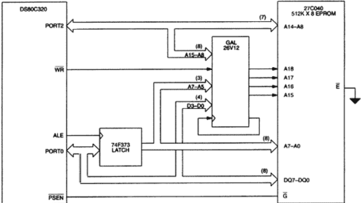
Figure 6. DS80C320 Latched Address Memory Hardware Example
